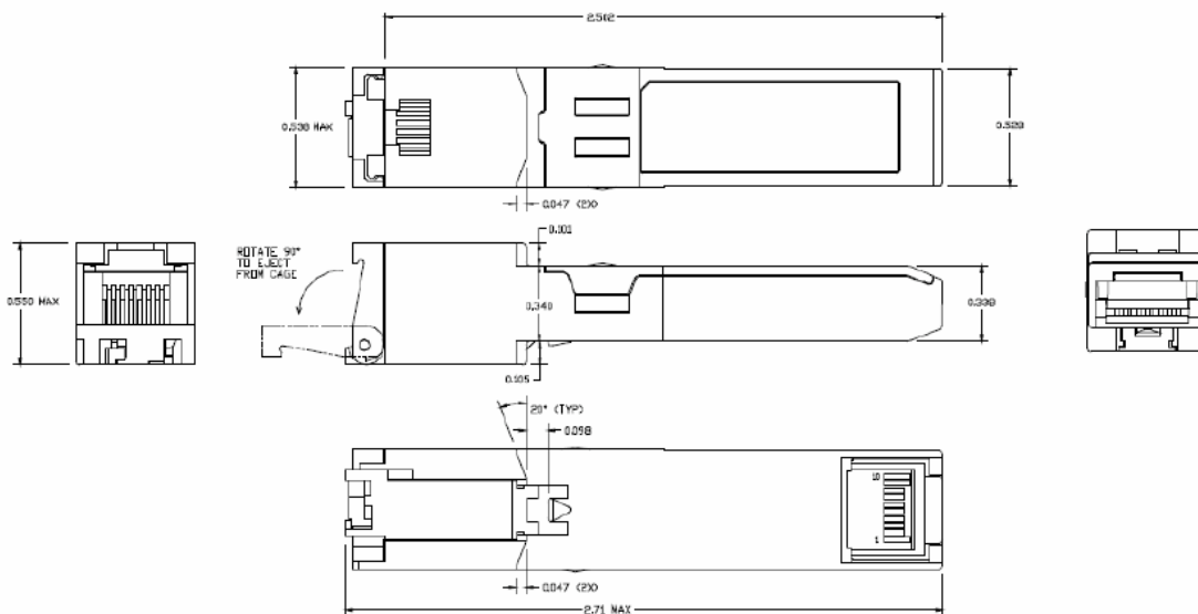
Figure 2. SFP-TX-01 mechanical dimensions
